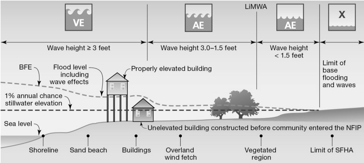
FIGURE 1 – TRANSECT SCHEMATIC
