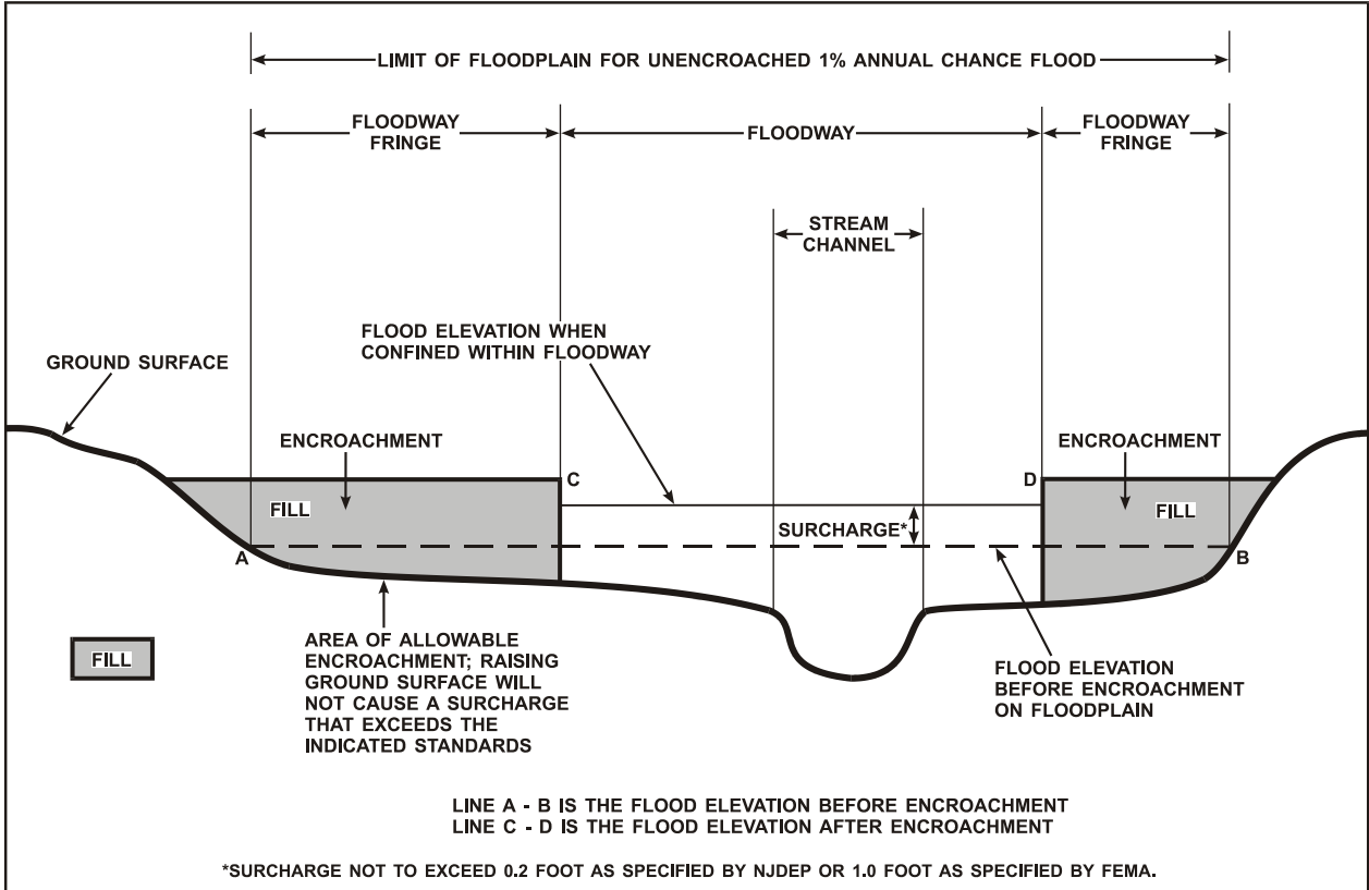
FIGURE 3 – FLOODWAY SCHEMATIC
